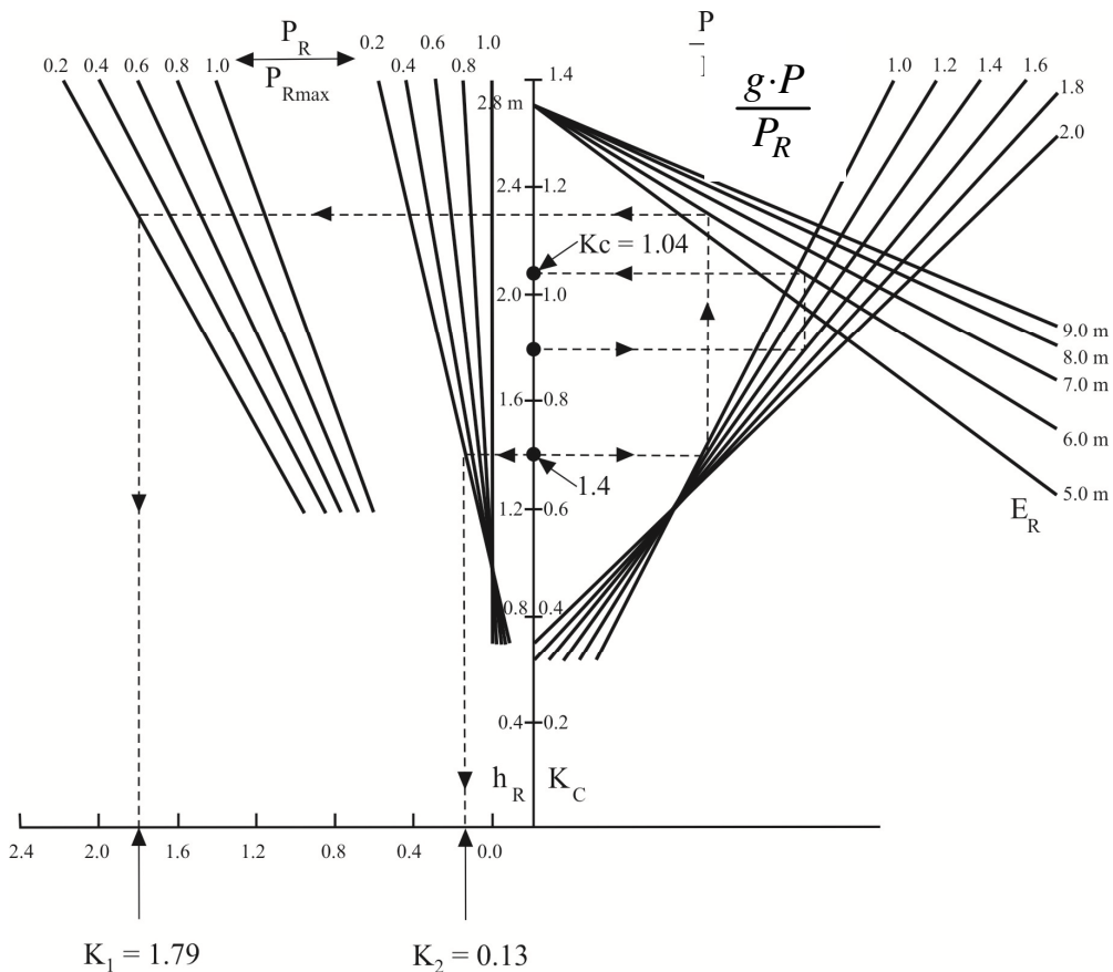
Diagram 4B (See paragraph 4. and diagram 4A of this annex)
