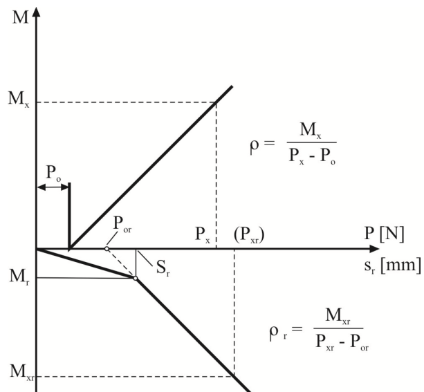
Figure 6 Mechanical Brake (See paragraph 2. of this annex)
