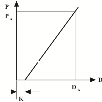
Figure 3 Hydraulic-transmission (See paragraphs 2.2.10. and 5.4.2. of this annex)
