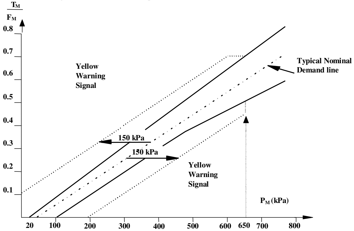
Diagram 2 Tractive units for semi-trailers
